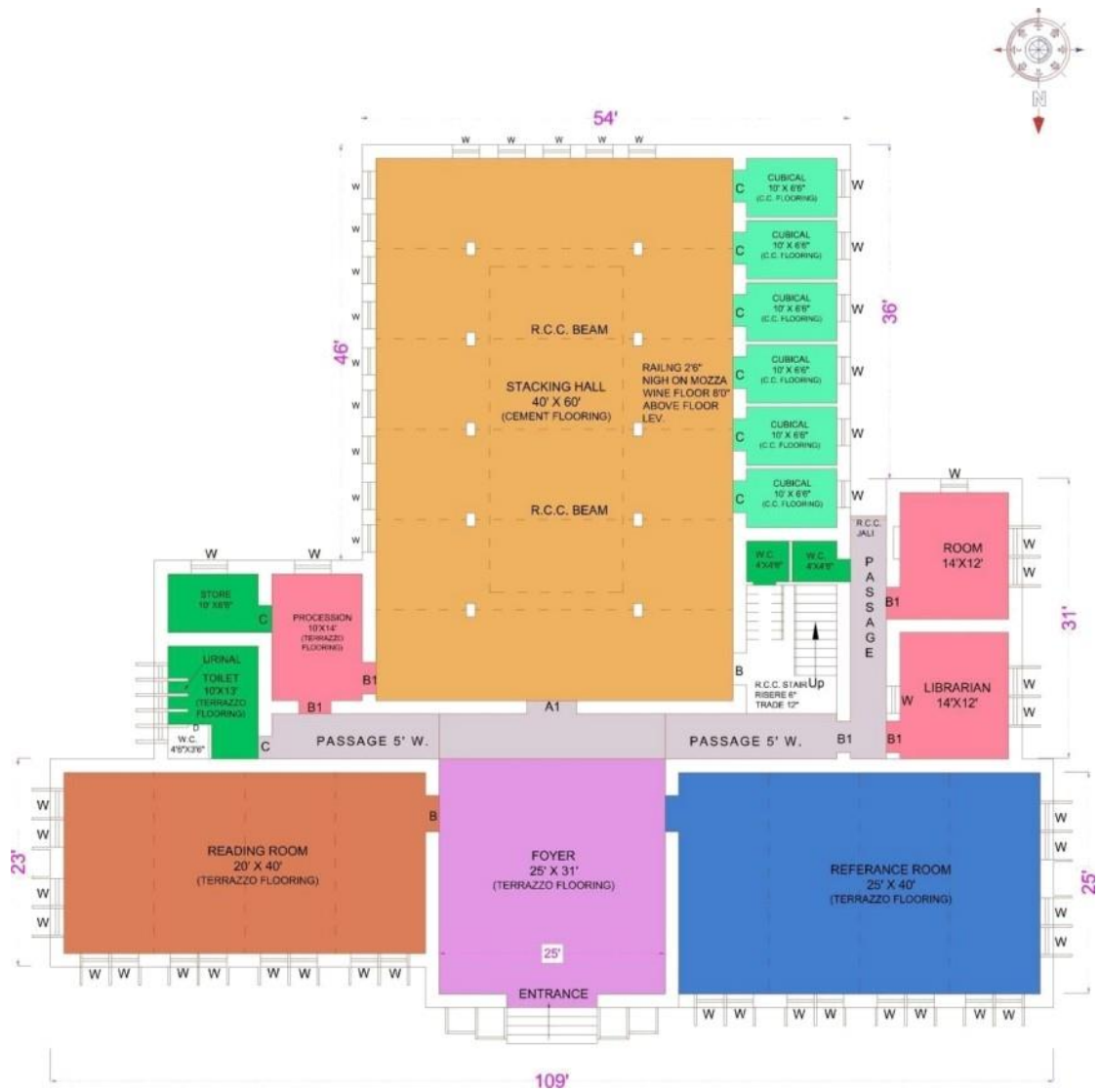
LIBRARY LINE PLAN
