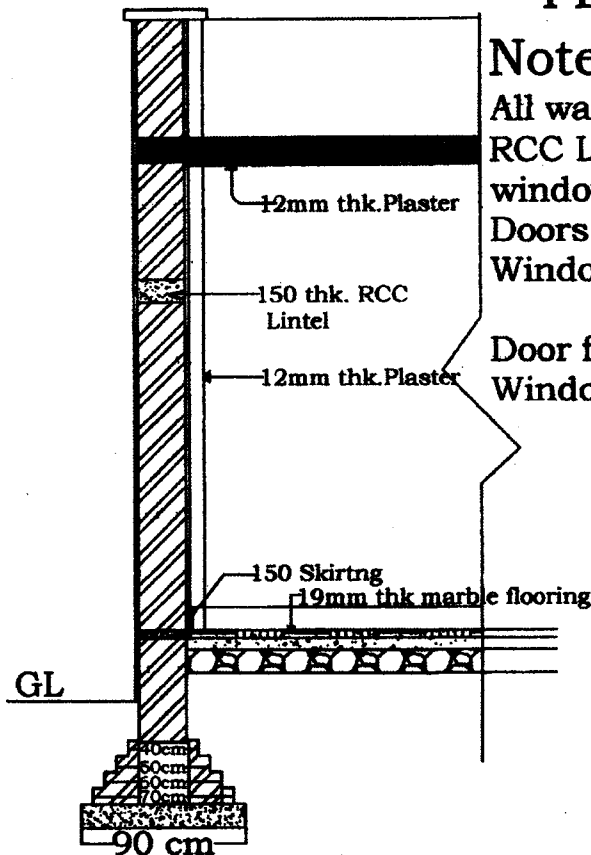
General Wall Section AA
